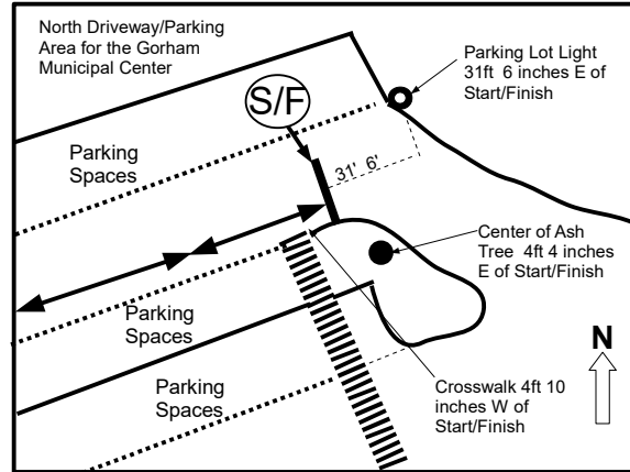
Start/Finish (S/F) Detail
